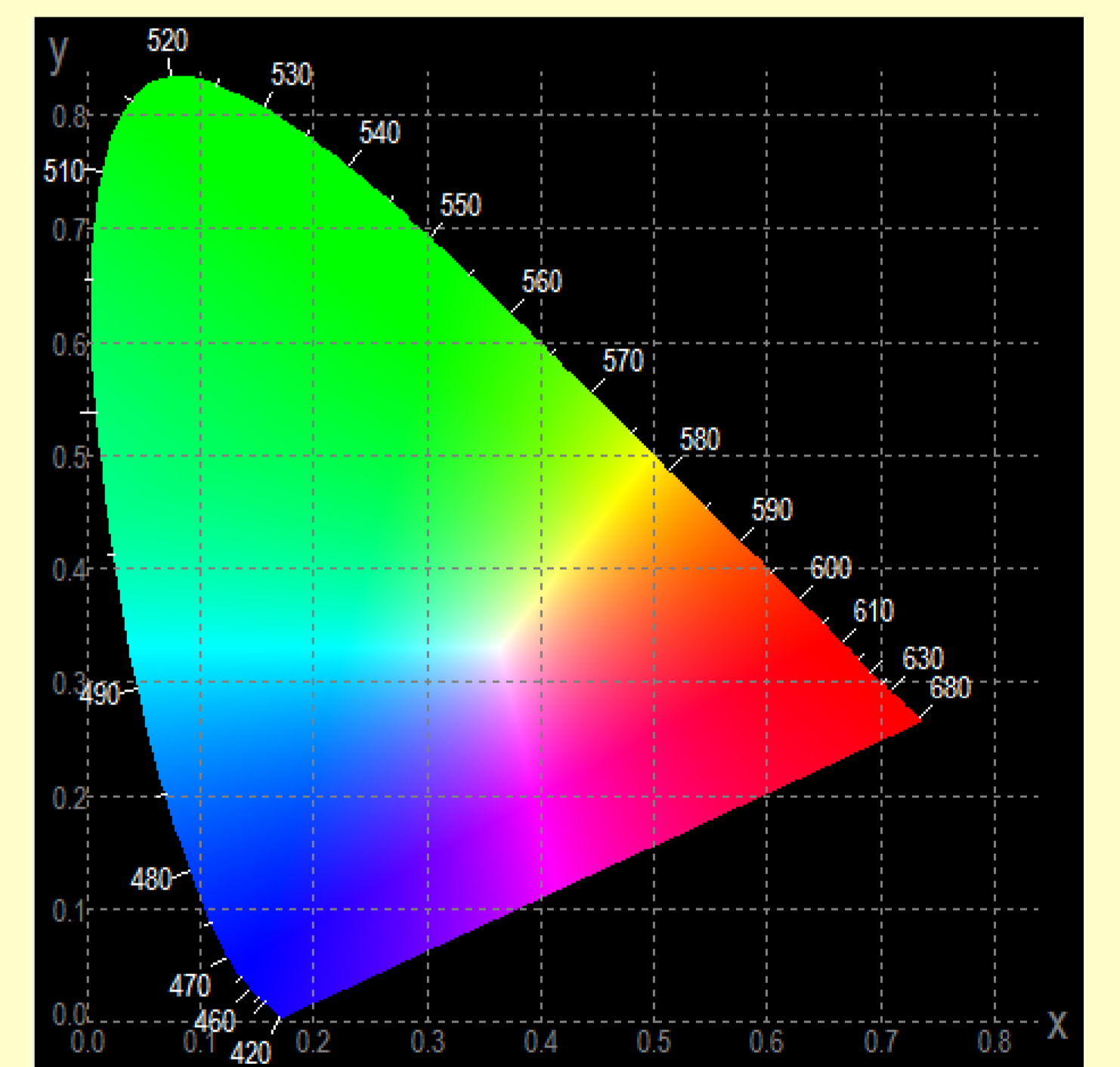
Right: the 1931 CIE chromaticity diagram developed from Maxwell's triangle
